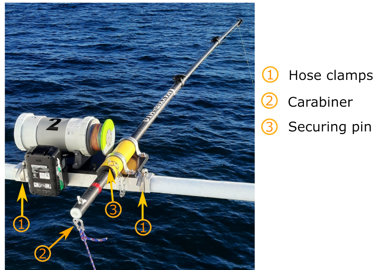
Figure 1. Winch unit installed on a ship's railing showing hose clamps, securing pin, and attachment carabiner.
